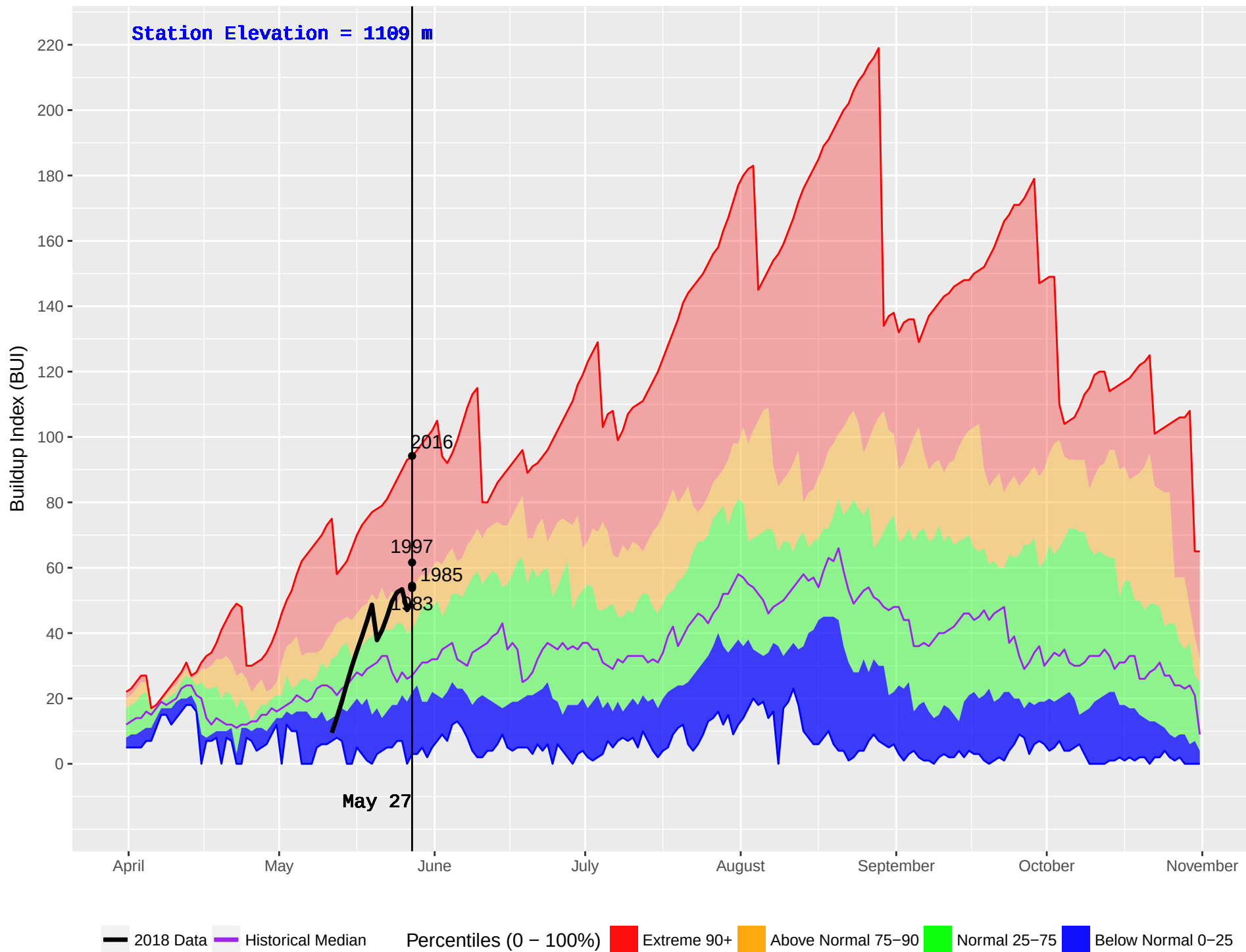
MOOSE LAKE (165) : Historical (1980–2016) and Current (2018) Noon Buildup Index (BUI)
