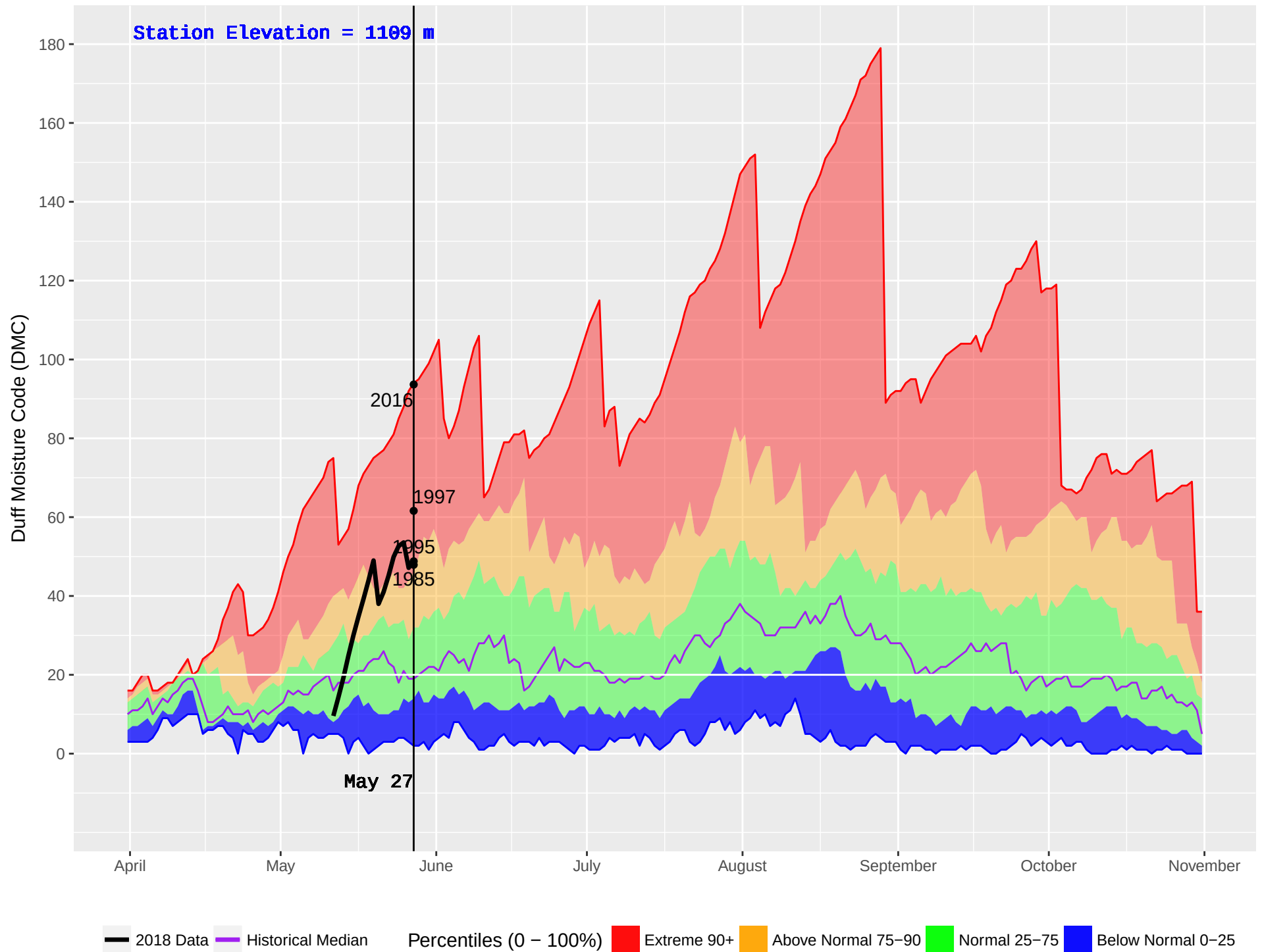
MOOSE LAKE (165) : Historical (1980–2016) and Current (2018) Noon Duff Moisture Code (DMC)
