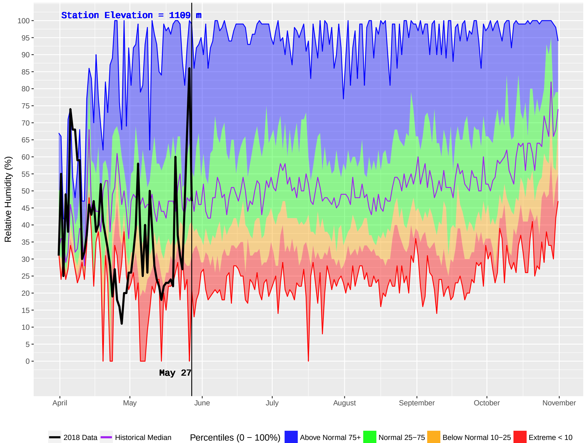
MOOSE LAKE (165) : Historical (1980–2016) and Current (2018) Noon Relative Humidity
