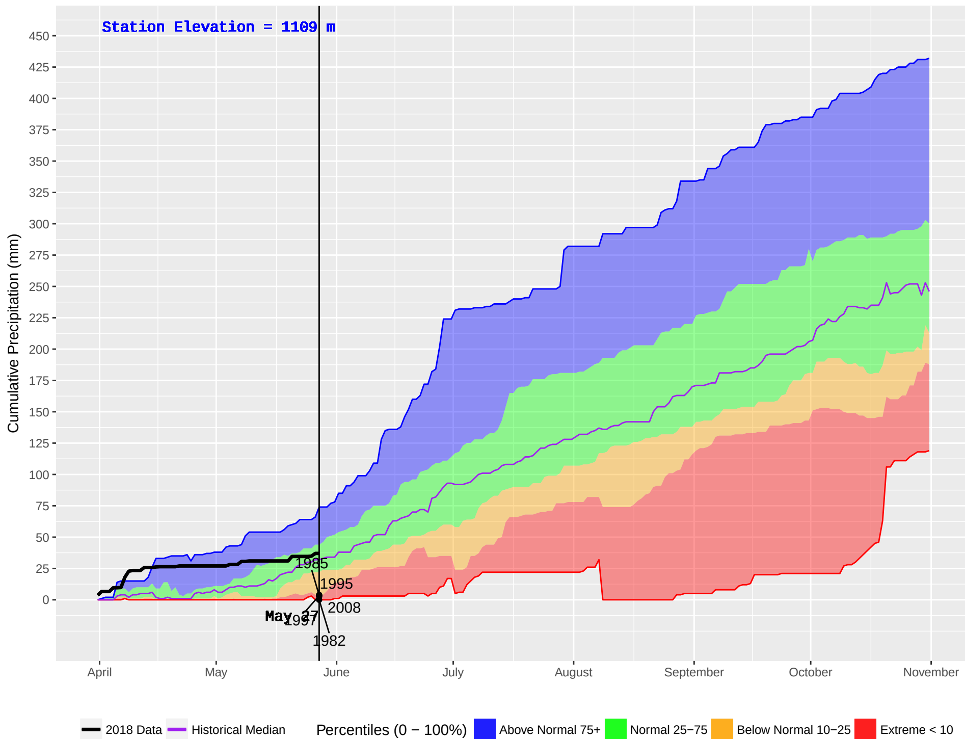
MOOSE LAKE (165) : Historical (1980–2016) and Current (2018) Noon Cumulative Precipitation
